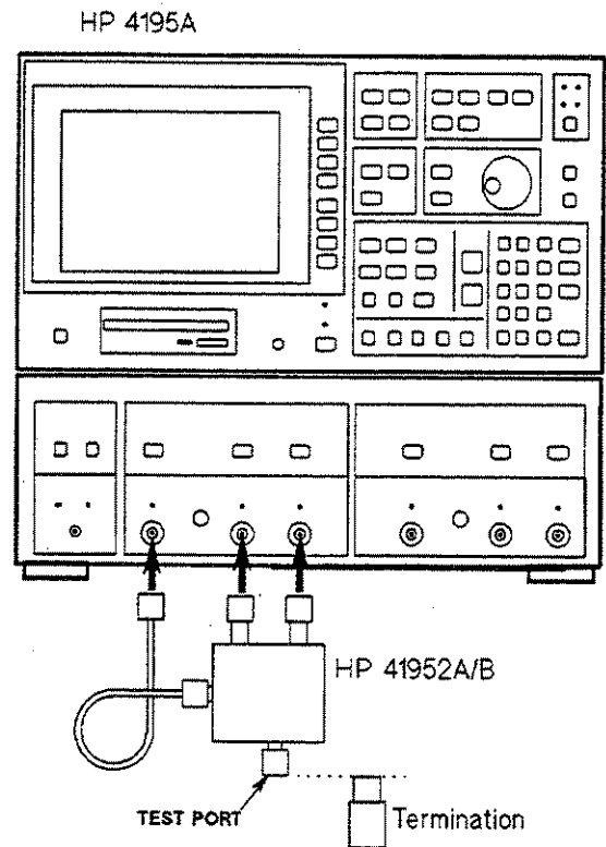
Figure 3-2. Operator's Check Setup
